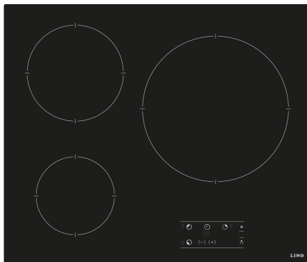
PL3 TCT3MAX S
